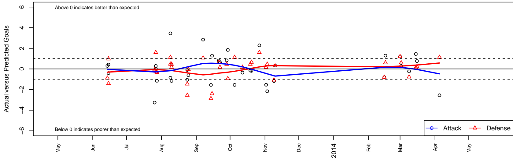
Crossfire OR SSC Freedom G00 Dots are actual minus expected GF (blue circles) and GA (red triangles). Blue line is smoothed change in attack strength. Red is smoothed change in defense strength.
